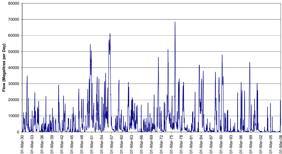
Flow in the Darling River at Wilcannia
